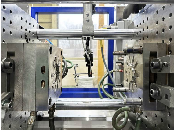
Fig. 3: Thanks to its servo drives, the WX90 offers highly precise, fluid movements.
